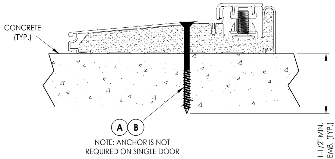
1 3 VERTICAL CROSS SECTION Inswing Threshold
